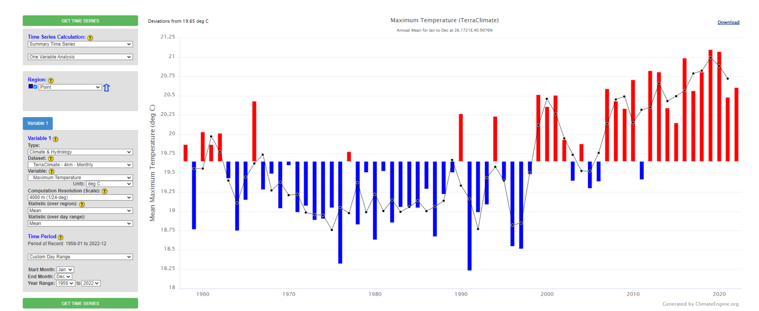
Historical data of the max temperature for the Feres area (1958-2022), exported from climateEngine app
