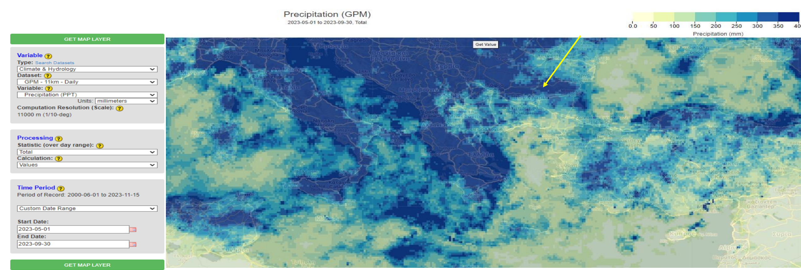
Precipitation (rainfall) data of the Feres area (2023 summer period), exported from climateEngine app
