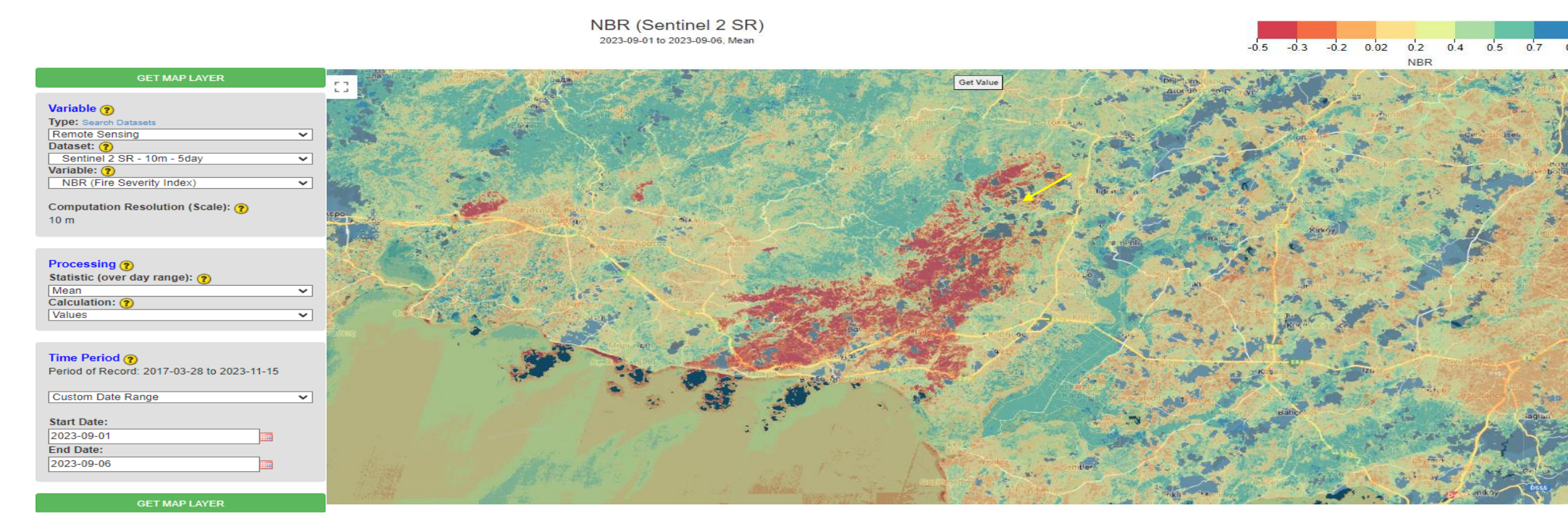
Fire index of the Feres area (September 2023), exported from climateEngine app
